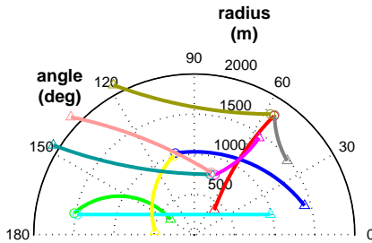
Fig. 7. Trajectories in the r\theta plane. Start/Stop positions for each track are shown with \circ/\triangle .
