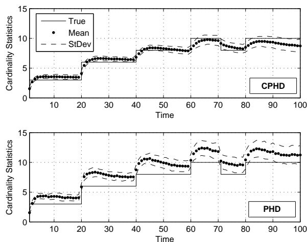
Fig. 5. 100 Monte Carlo run average results for CPHD and PHD filters for unknown detection probability. True and estimated target numbers for CPHD (top) and PHD (bottom).
