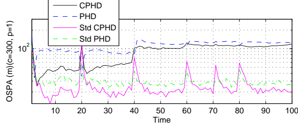
Fig. 6. OSPA miss distance versus time for the CPHD and PHD filters for unknown detection probability.
