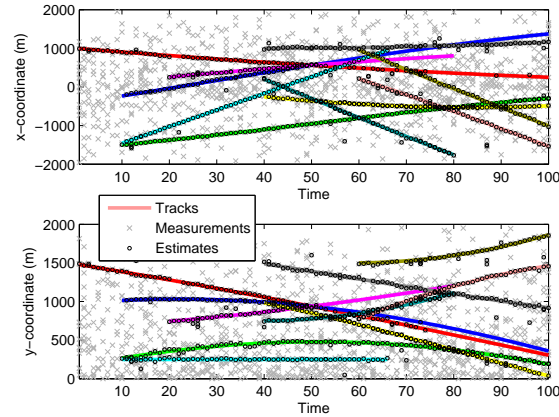
Fig. 8. Unscented Kalman CPHD filter for jointly unknown clutter rate and detection probability: filter estimates and true tracks in x and y coordinates versus time
