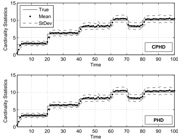
Fig. 2. 100 Monte Carlo run average results for CPHD and PHD filters for unknown clutter rate. True and estimated target numbers for CPHD (top) and PHD (bottom).
