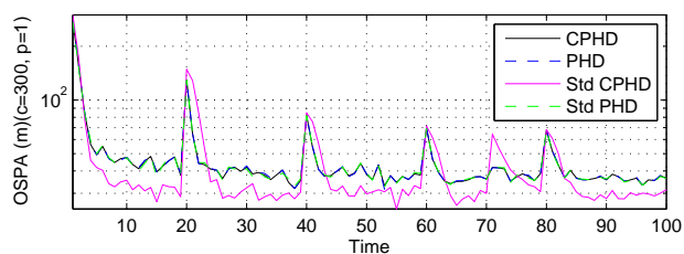
Fig. 4. OSPA miss distance versus time for the CPHD and PHD filters for unknown clutter rate.
