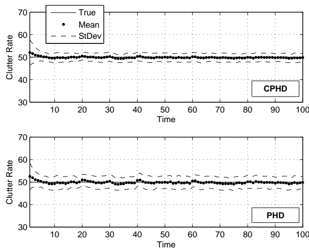
Fig. 3. 100 Monte Carlo run average results for CPHD and PHD filters for unknown clutter rate. True and estimated mean clutter rate for CPHD (top) and PHD (bottom).
