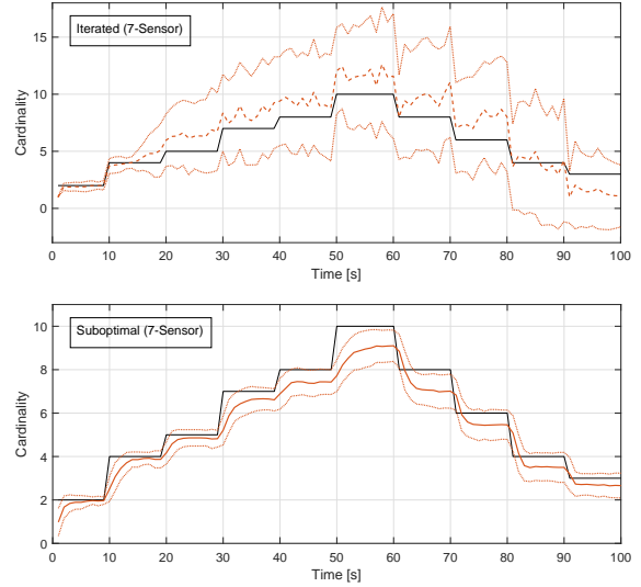
Fig. 5. 7-sensor case: true and mean cardinality (with 1-sigma bounds).
