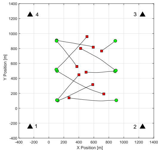
Fig. 1. Scenario 1: ground truth and sensor layout. The triangles ( \blacktriangle ) are the locations of bearing-only sensors, the green circles ( \bullet ) indicate the object starting positions, and the red squares ( \blacksquare ) are the final positions.
